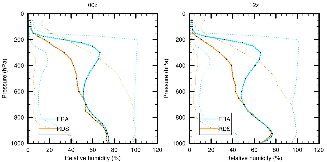
Figure 6. Example of profile-comparison of the soundings (RDS) and ERA-Interim from location De Bilt. Average, 5 and 95 percentile of the parameter relative humidity in spring (months MAM) 00 and 12 UTC
